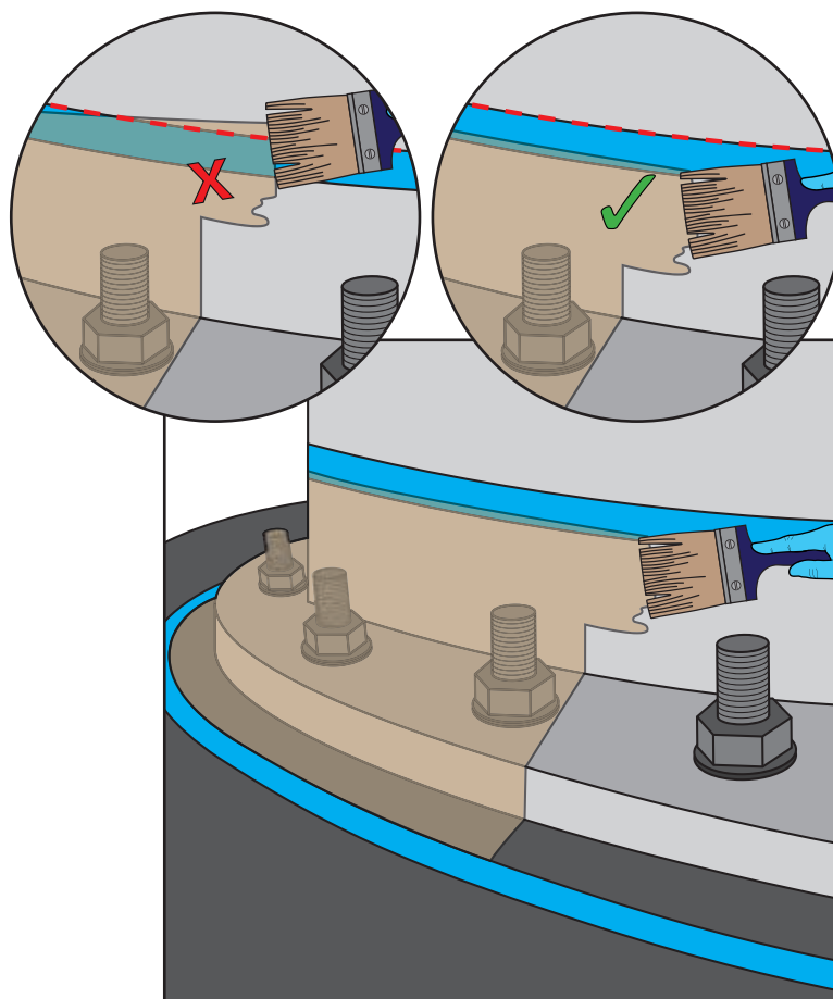
Fig. 2: Apply the Hi-Tack Primer, ensuring not to contaminate any areas outside of the masking tape (inset).
