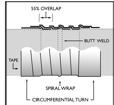
Fig. 13: Note method of wrapping. 1. Start with one circumferential turn onto factory coating. 2. Then change to spiral wrap with 55% overlap over weld area. 3. Finish with one circumferential turn over factory coating the opposite side of the weld. Overlap tape at least 75mm onto existing coating. 4. Circumferential wrap of Denso PVC Self-Adhesive Tape can be added, as (A) .
