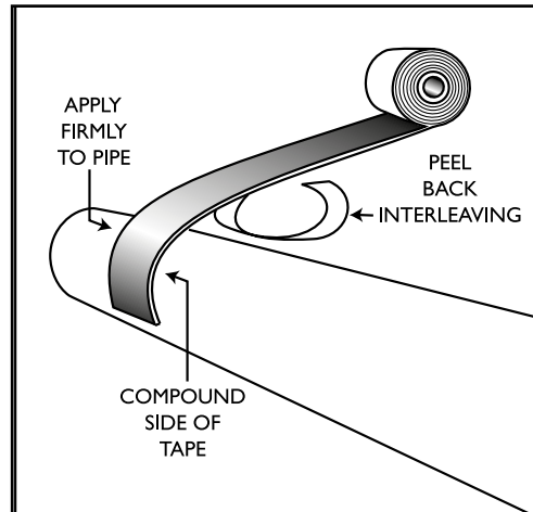
Fig. 4: Starting the first roll of tape.
