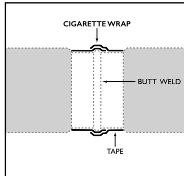
Fig. 12: If the factory coating is 3LPE, the typical thickness can be between 2.5mm to 5mm. It is therefore important to chamfer the edge of the 3LPE to 35°. Denso Primer D should be applied to the entire joint and onto the 3LPE by at least 75mm. Densopol Tape should then be applied using a cigarette method to completely cover the joint and factory cutback. The ends of the cigarette wrap should overlap by the same distance as the width of the tape being used.
