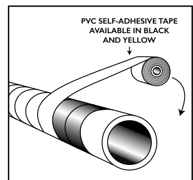
Fig. 10: Apply an optional outerwrap of Denso PVC Self-Adhesive Tape with 55% overlap, beginning and ending the wrap with two full circumferential turns.
