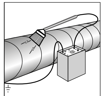
Fig. 24: Perform a holiday test using a ring or brass brush (refer to the table for holiday detection voltages).
