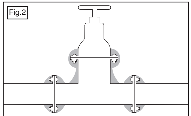
Fig. 2. Fill all voids with Denso Profiling Mastic and build up the profile around the valve flanges and shoulders so that there are no sharp angles.
